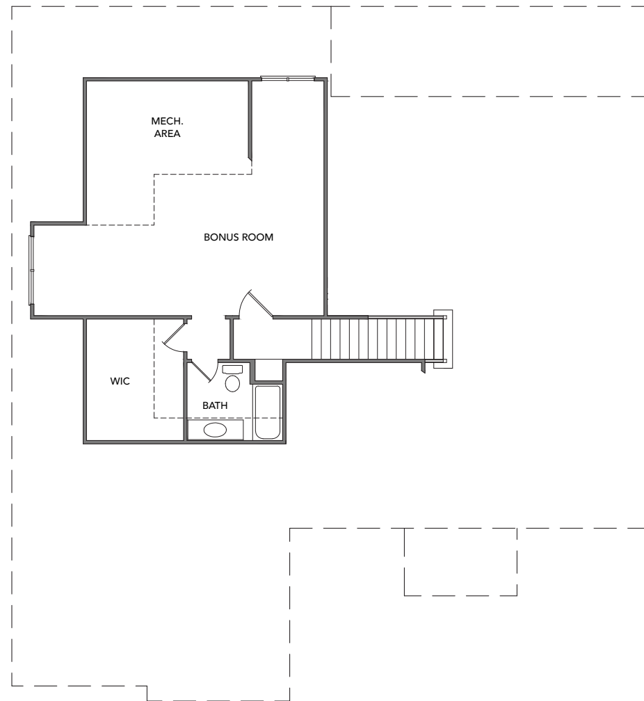
SECOND FLOOR
